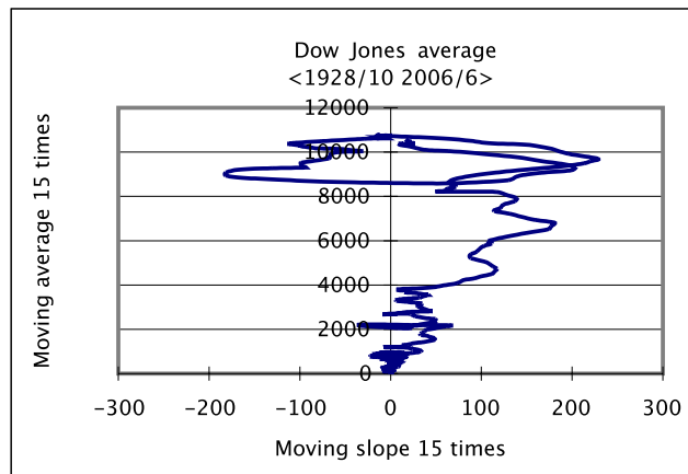
Figure 8. Point of forecast on a one-dimensional phase diagram.
